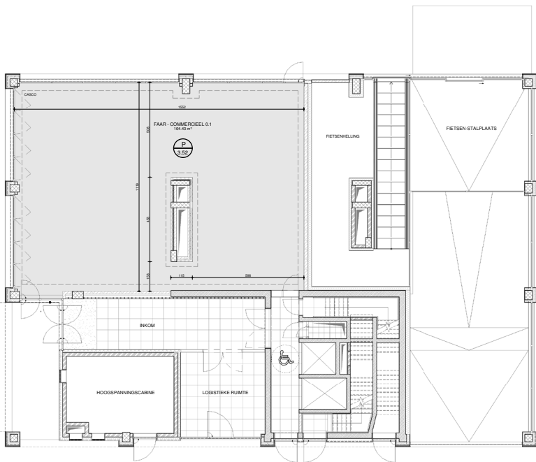
Verdieping +00
